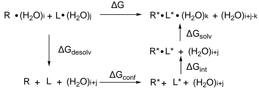
Figure 1.1. The process of a ligand binding to a receptor. R represents the receptor; L represents the ligand; i is the number of water molecules inside the binding pocket of the receptor; j is the number of the water molecules surrounding the ligand; k is the number of the water molecules left in the binding pocket when the ligand is bound. * indicates the conformational change associated with binding. desolv, conf, int and solv indicate the desolvation, conformational change, interaction and solvation respectively.
